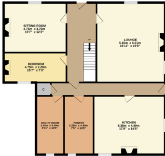
GROUND FLOOR 123.5 sq.m. (1329 sq.ft.) approx.
